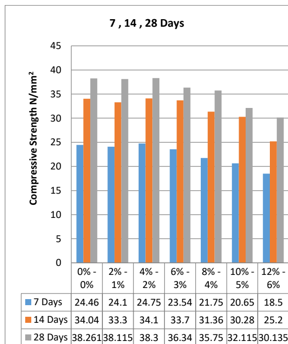
Figure 6: Replacement Percentage of Cement with Marble Dust Powder and Coconut Fiber, After 7, 14, 28 Days Compressive Strength
