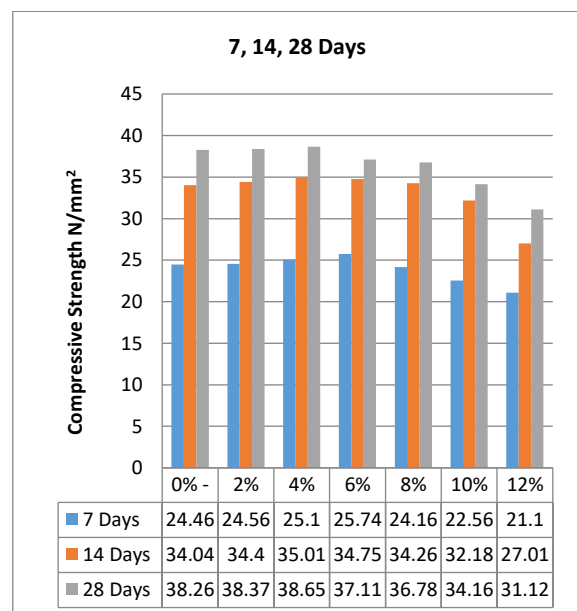
Figure 5: Replacement Percentage of Marble Dust Powder, After 7, 14, 28 Days Compressive Strength
