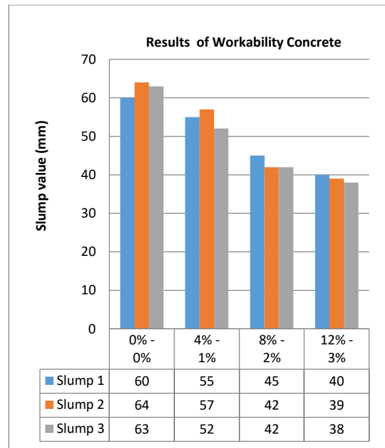
Figure 7: Shows the Slump Value of Trial Mix Different Percentage
